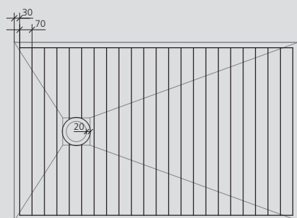
Fundo Slim 1600 × 1000 mm
