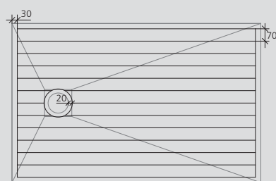
Fundo Slim 1400 × 900 mm
